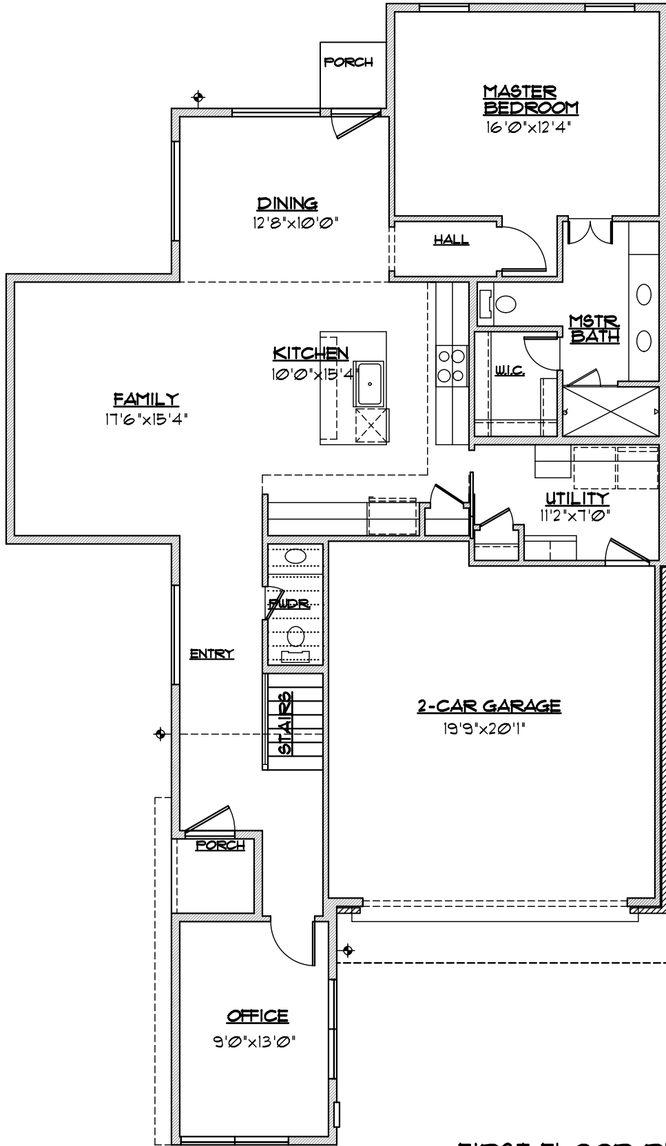
FIRST FLOOR PLAN 1/8" = 1'0"
